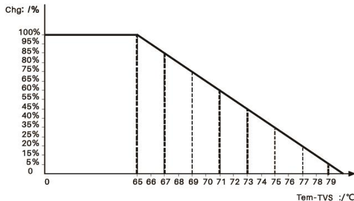
Fig. 5-1 When the ambient temperature rises higher than the set value, the controller will stop charging and discharging.
