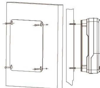
Fig. 2.1 Installation and heat dissipation
